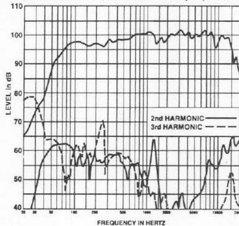
FIGURE 6 — Harmonic Distortion, 0.1 Rated Power Input (10 watts)
