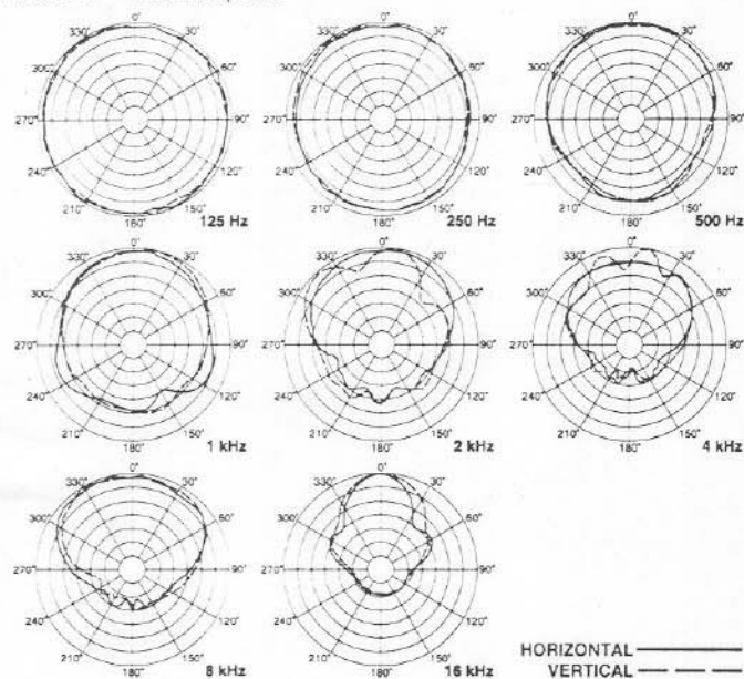
FIGURE 2 — Polar Response
