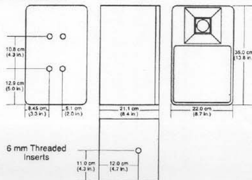
FIGURE 8 — Dimensions
